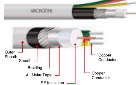
Cross Section View for 3+1 CCTV
