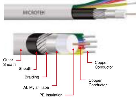
Cross Section View for 4+1 CCTV
